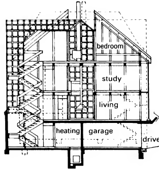
④ Section
